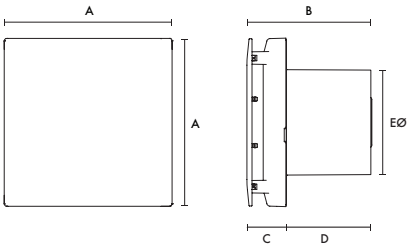
Closed Grille
