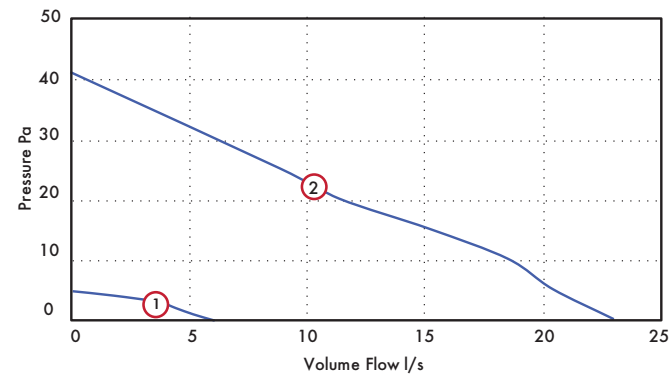
Open Grille
